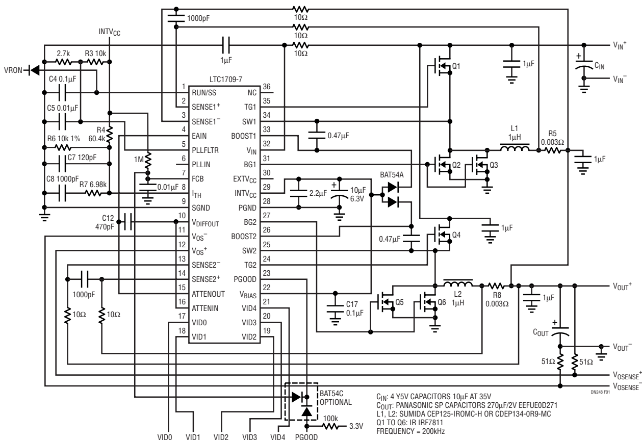
Figure 1. Schematic Diagram of a 25A Mobile VRM
